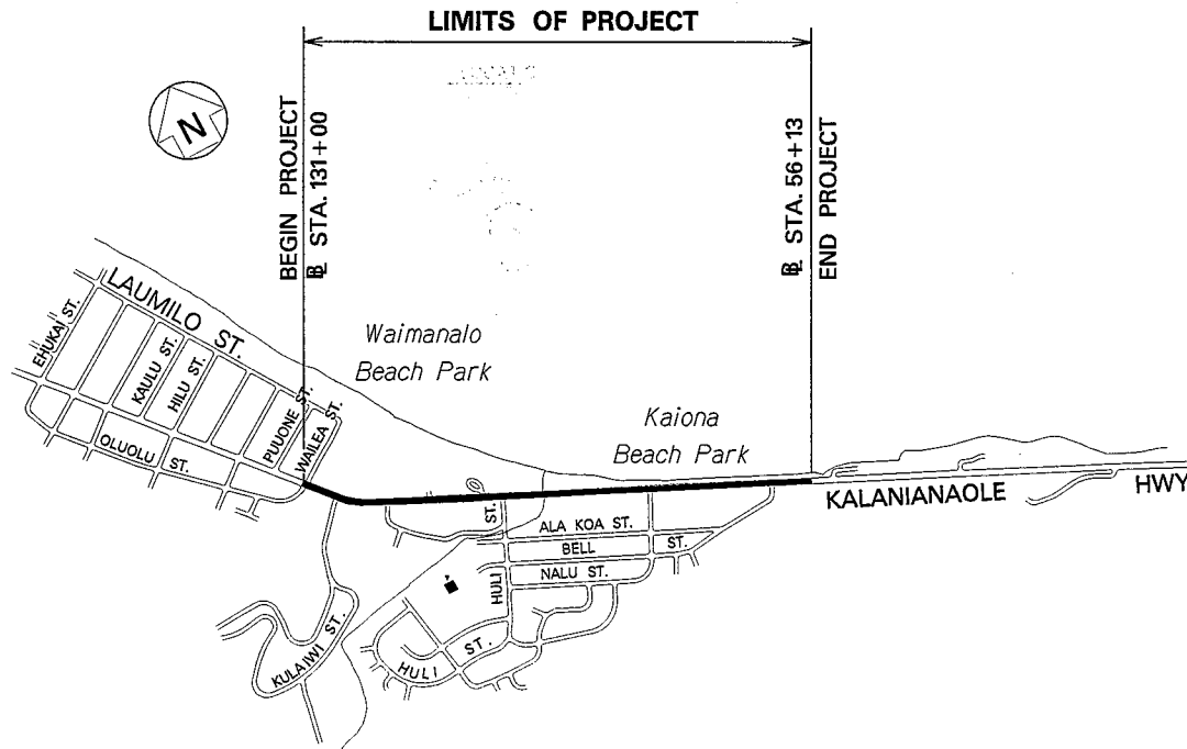
LAYOUT PLAN
