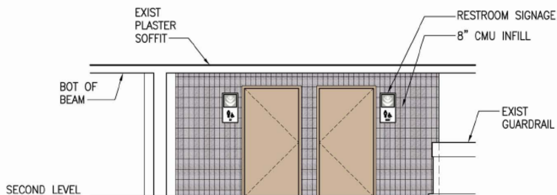
EXTERIOR ELEVATION C/A1-201 SCALE: 1/4"=1'-0"
