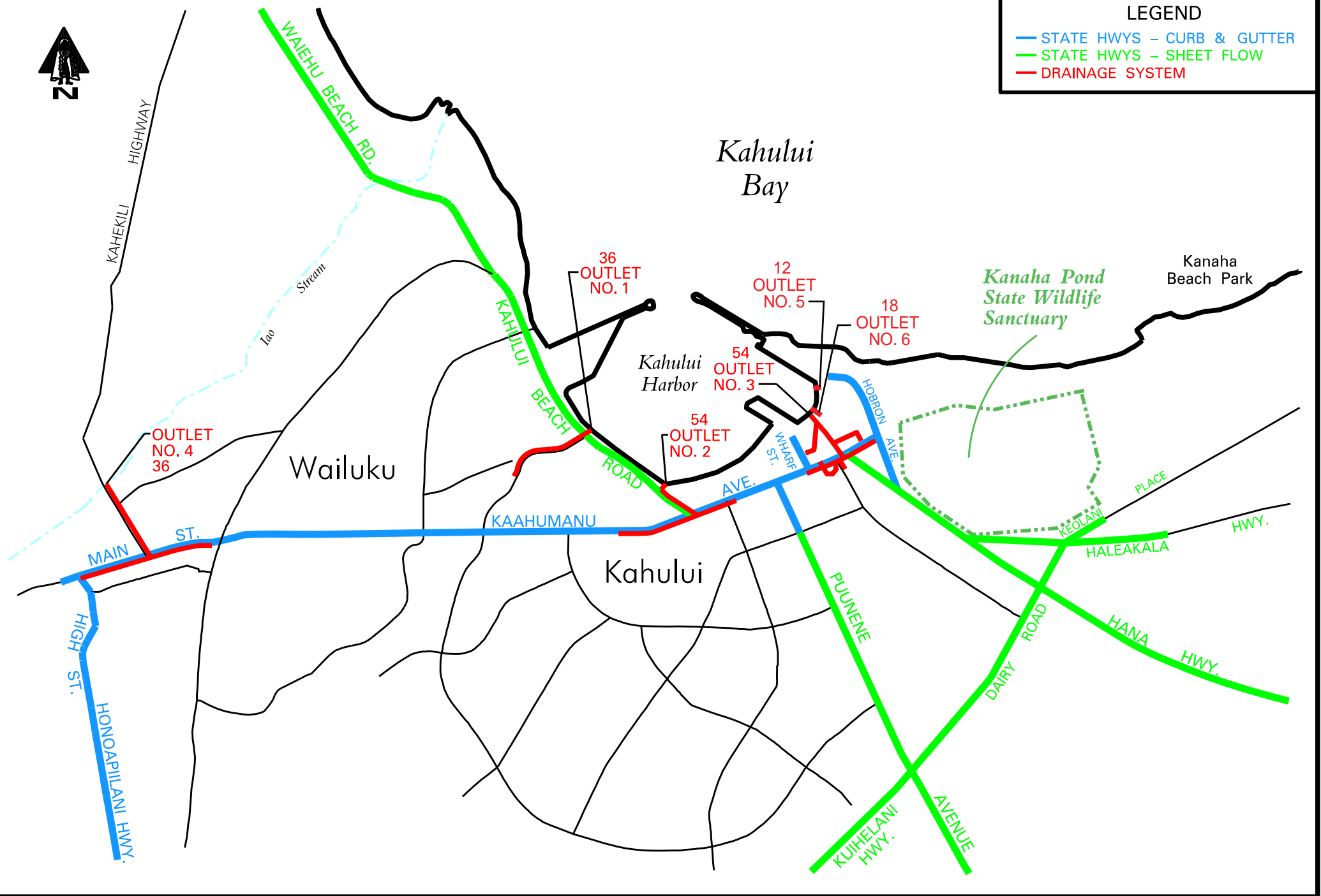
ATTACHMENT A.2 — MAJOR STORM DRAIN SYSTEM (WAILUKU — KAHULUI)
