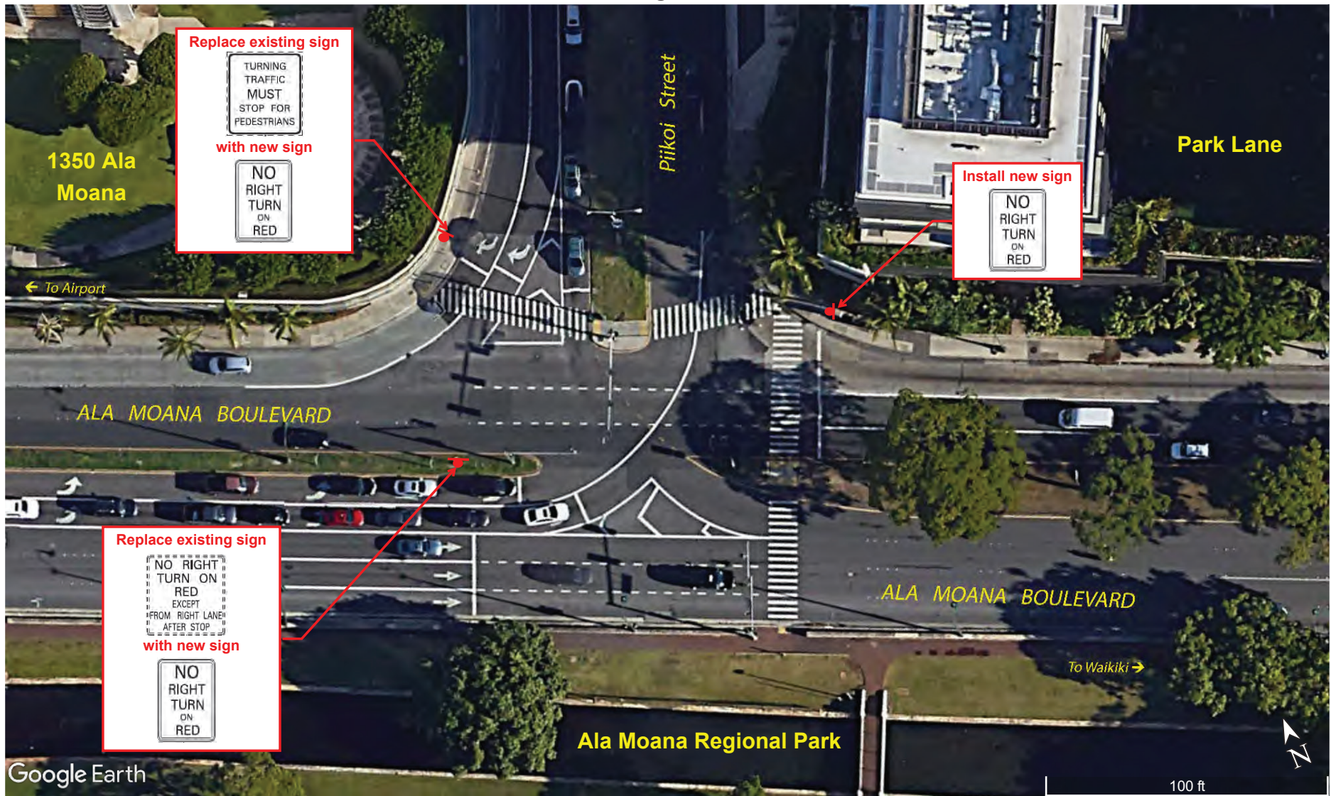
Piikoi Street Intersection Improvements
