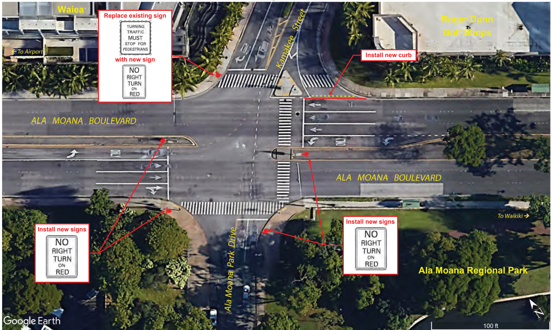
Kamakee Street Intersection Improvements
