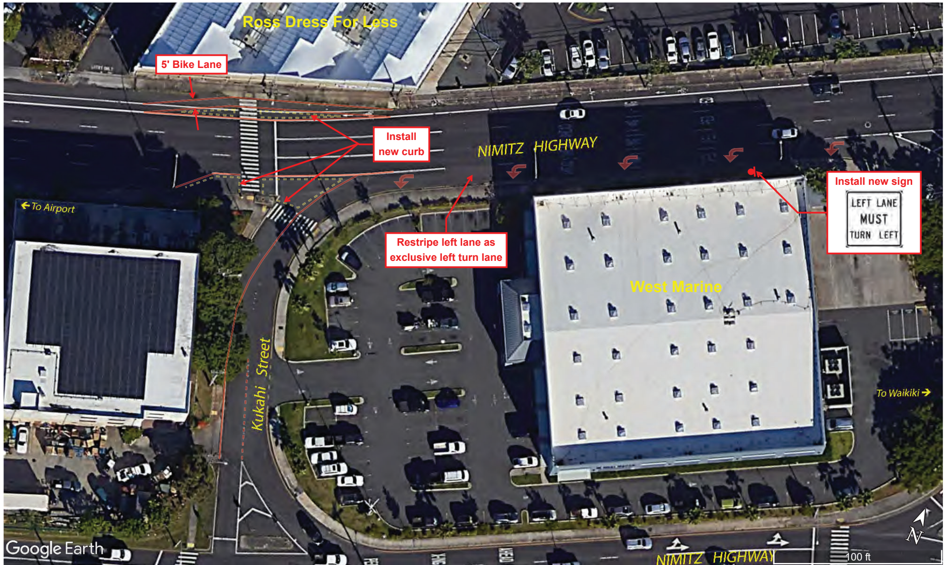
Kukahi Street Improvements
