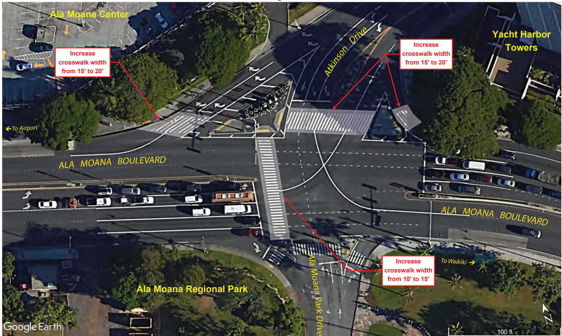
Atkinson Drive Intersection Improvements
